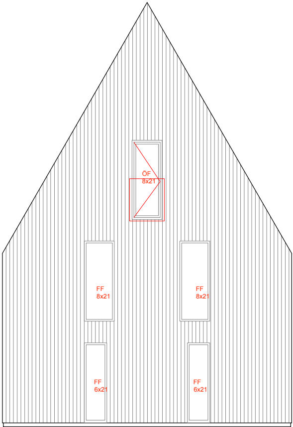
GAVELFASAD (norr)
